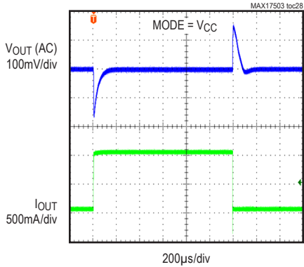
MAX17503 3.3V OUTPUT, DCM MODE (LOAD CURR STEPPED FROM 50mA TO 1A), FIGURE 4b CIRCUIT
