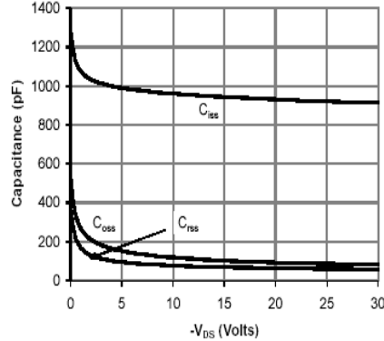
Figure 8: Capacitance Characteristics
