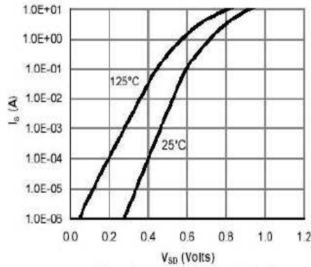
Figure 6: Body-Diode Characteristics
