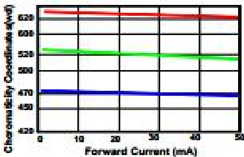
7). Wavelength and current
