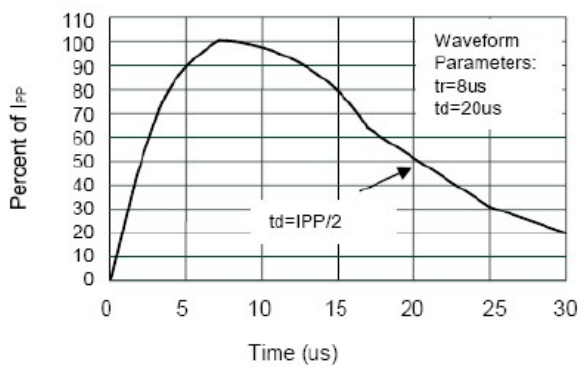
Pulse Waveform
