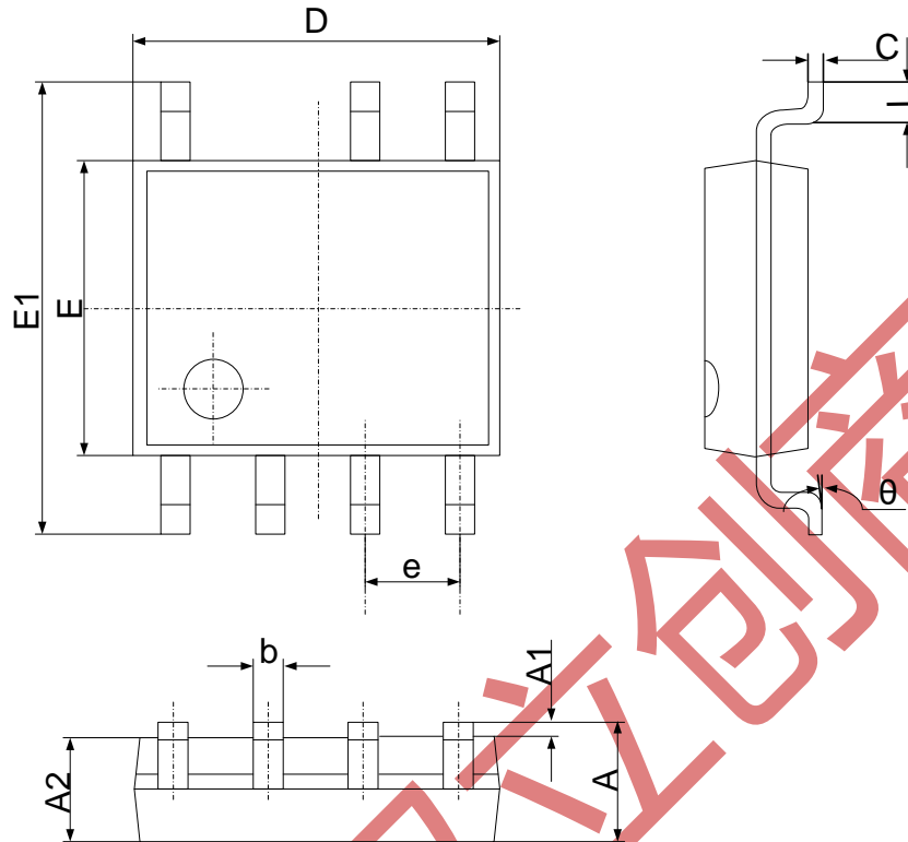
SOP-7
