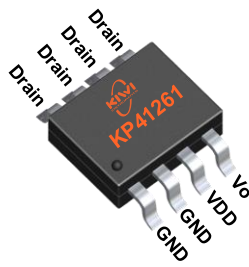
SOP-8
