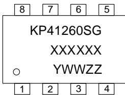
SOP-8
