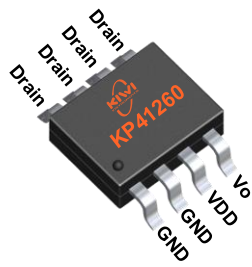
SOP-8
