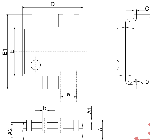
SOP-7
