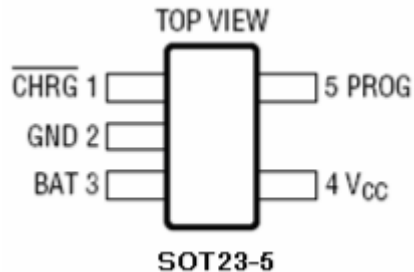
Figure 2. PIN Configuration
