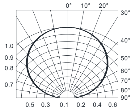
Fig.6-Radiation Diagram Ta=25°C
