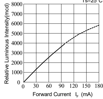
Fig.2-Relative Luminous Intensity vs. Forward Current Ts=25°C
