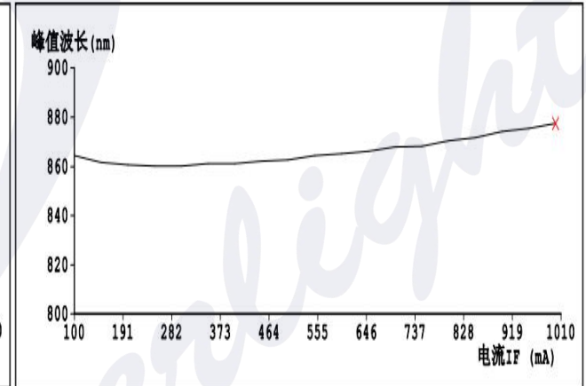
Spectral wavelength
