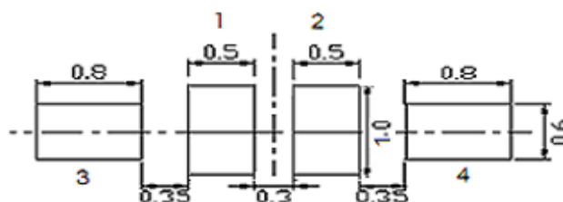
Recommended Soldering Pattern (Units : mm).
