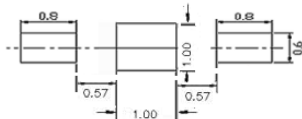
Recommended Soldering Pattern (Units : mm)-
