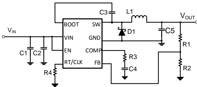
4.5V-50V, Asynchronous Buck Converter
