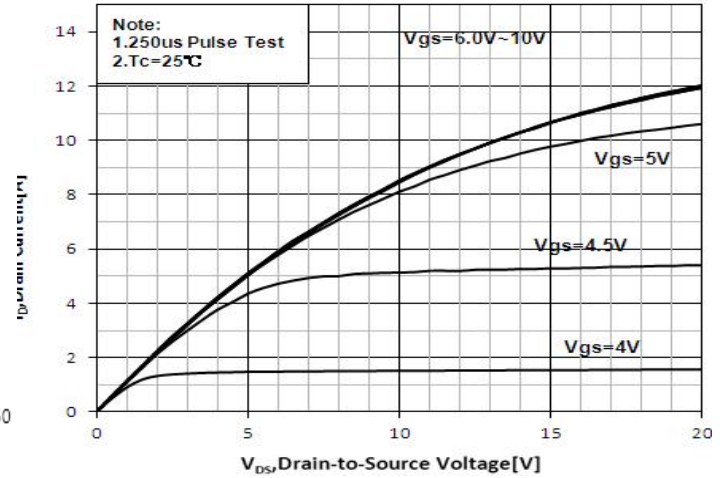
Figure 2 Typical Output Characteristics
