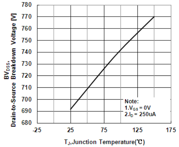
Figure 9 Typical Breakdown Voltage vs Junction Temperature
