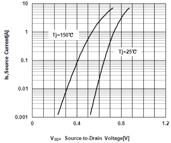
Figure 5 Typical Body Diode Transfer Characteristics
