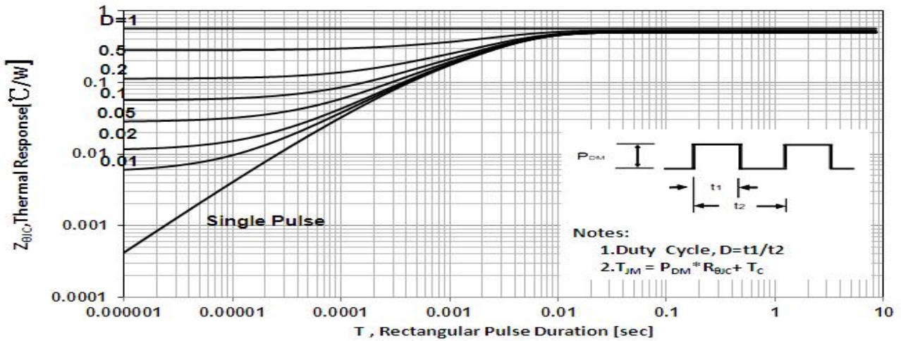
Figure 3 Maximum Effective Thermal Impedance , Junction to Case
