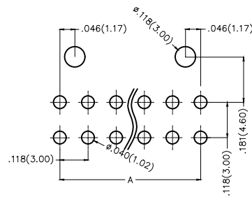
8~20 Circuits
