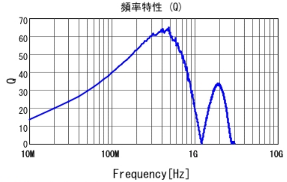
■ LQW2BASR12J00 Q
