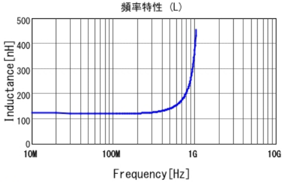
■ LQW2BASR12J00 L
