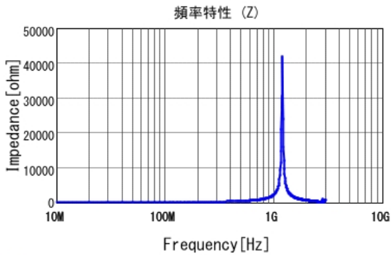
■ LQW2BASR12J00 |Z|
