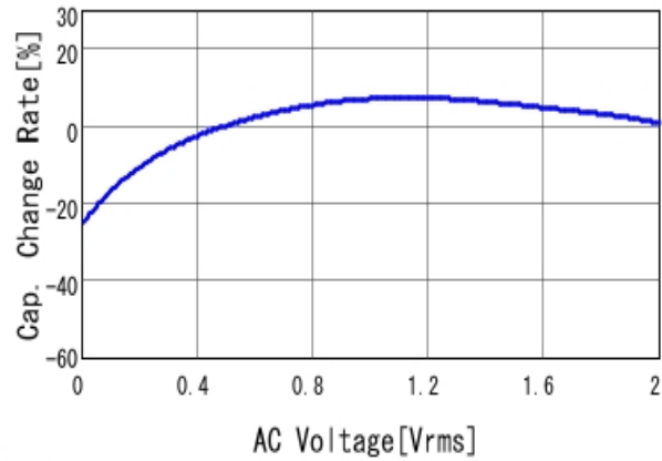
■ GRM188C80J106MEA6 C-AC Voltage capchange, DCOV, 25.0d
