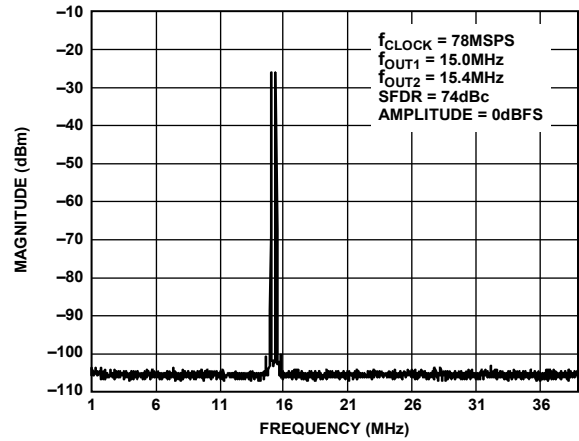
Figure 42. Dual-Tone SFDR
