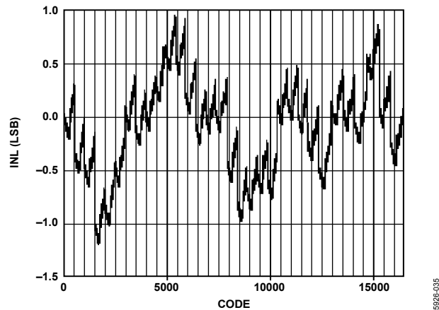
Figure 38. Typical Uncalibrated INL
