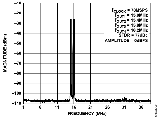
Figure 26. Four-Tone SFDR
