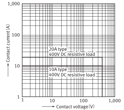
2.-(1) Max. value for switching capacity (10A and 20A types)
