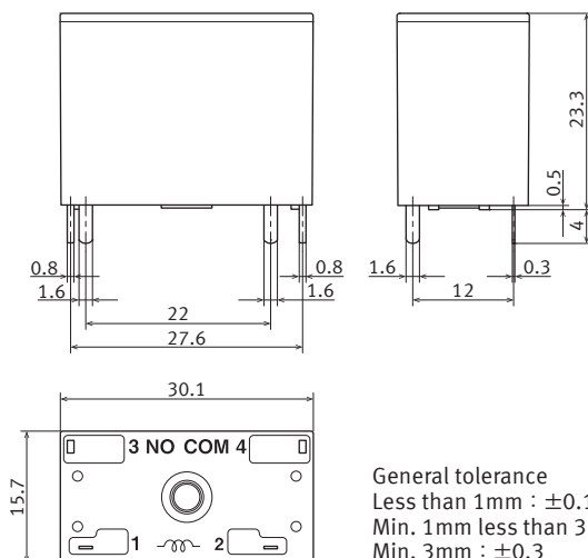
External dimensions
