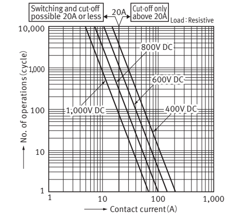
3.-(2) Switching life and cut-off curves (20A type)
