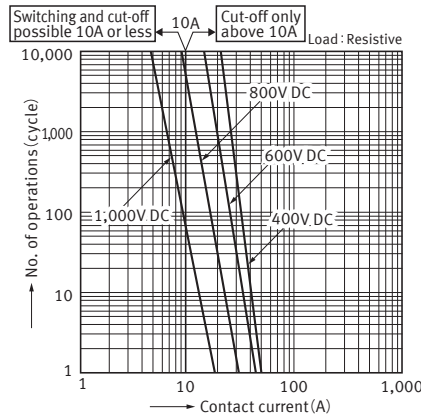
3.-(1) Switching life and cut-off curves (10A type)
