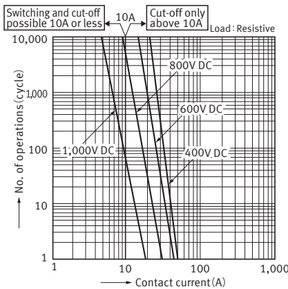
3.-(1) Switching life and cut-off curves (10A type)
