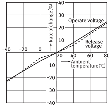
1.-(1) Ambient temperature characteristics (10A type)
