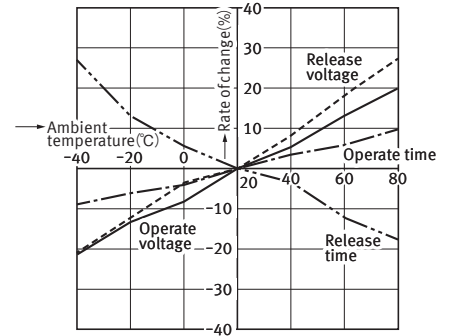
1.-(3) Ambient temperature characteristics (80A type)
