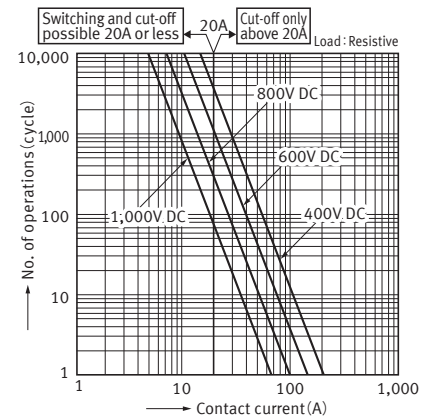
3.-(2) Switching life and cut-off curves (20A type)
