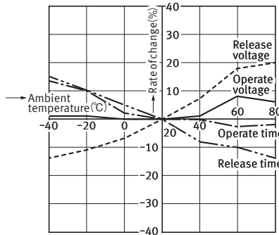
1.-(5) Ambient temperature characteristics (300A type)
