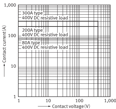
2.-(2) Max. value for switching capacity (80A, 200A and 300A types)
