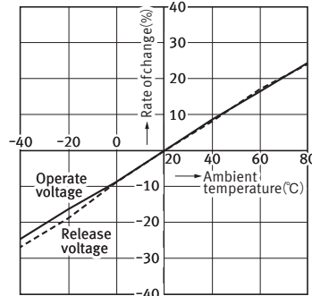
1.-(2) Ambient temperature characteristics (20A type)
