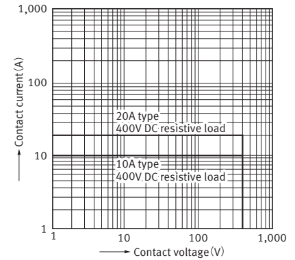
2.-(1) Max. value for switching capacity (10A and 20A types)
