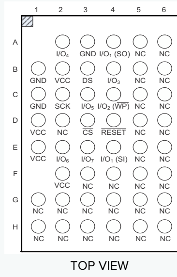
Figure 2-2. 46-ball WLCSP Pinout
