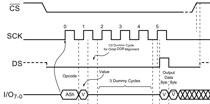
Figure 12-23. Echo with Inversion in Octal Mode — DDR
