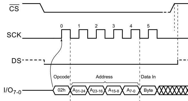
Figure 8-2. Byte Program in Octal Mode — SDR
