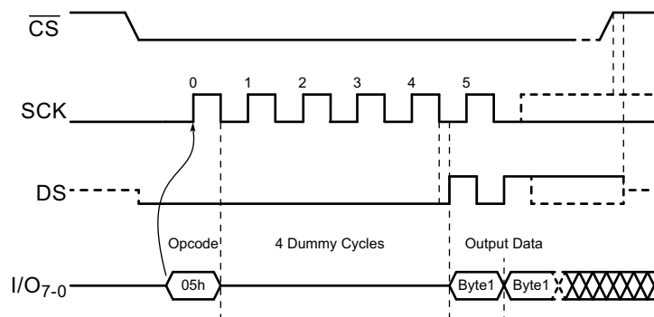
Figure 11-5. Read Status Register Byte 1 in Octal Mode — SDR
