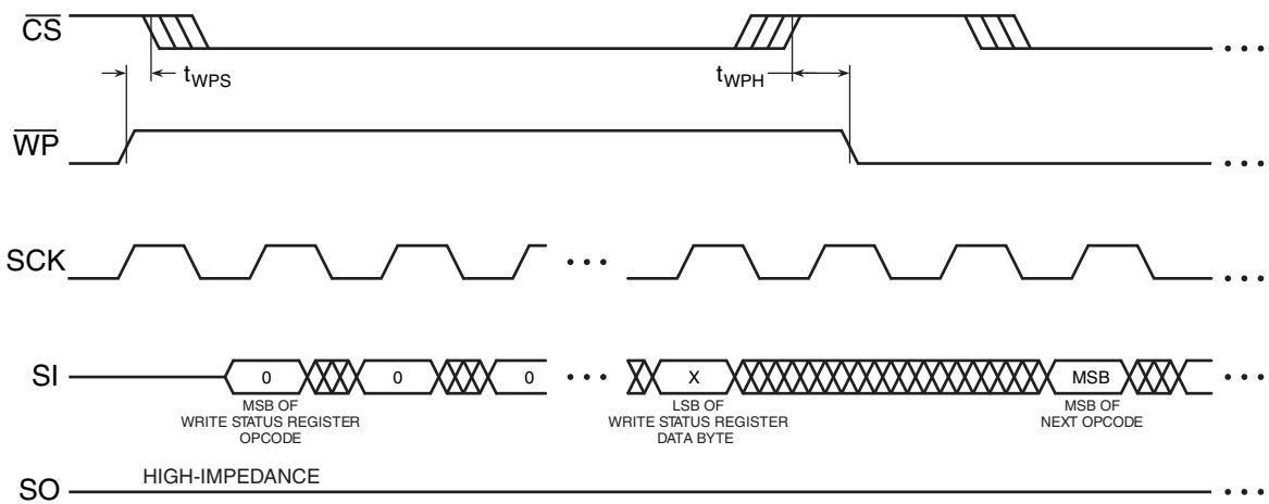
Figure 15-3. \overline{WP} Timing for Write Status Register Command
