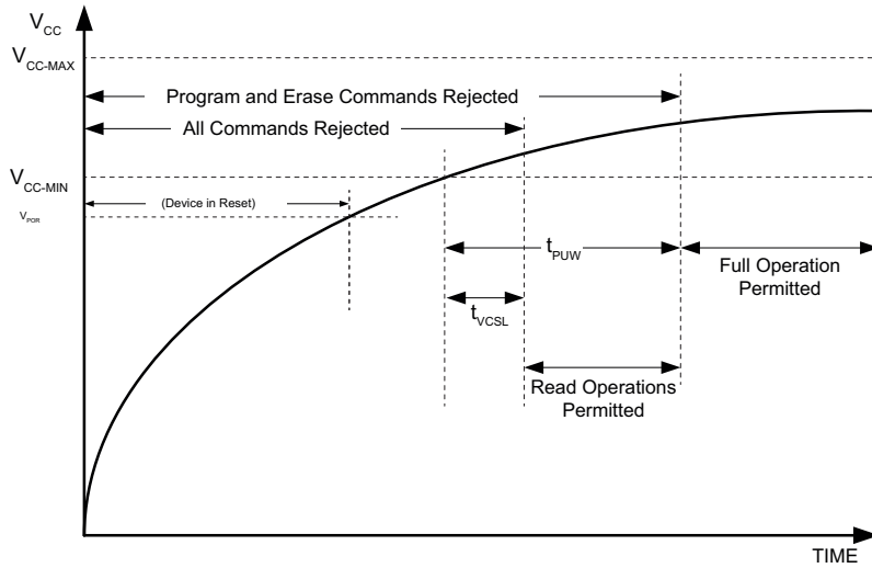
Figure 14-2. Power-Up After Brown-Out Timing
