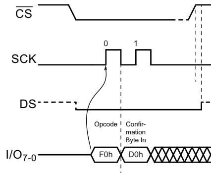
Figure 12-12. Reset (Terminate Operation) in Octal Mode —SDR
