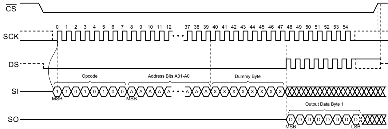
Figure 7-14. Buffer Read
