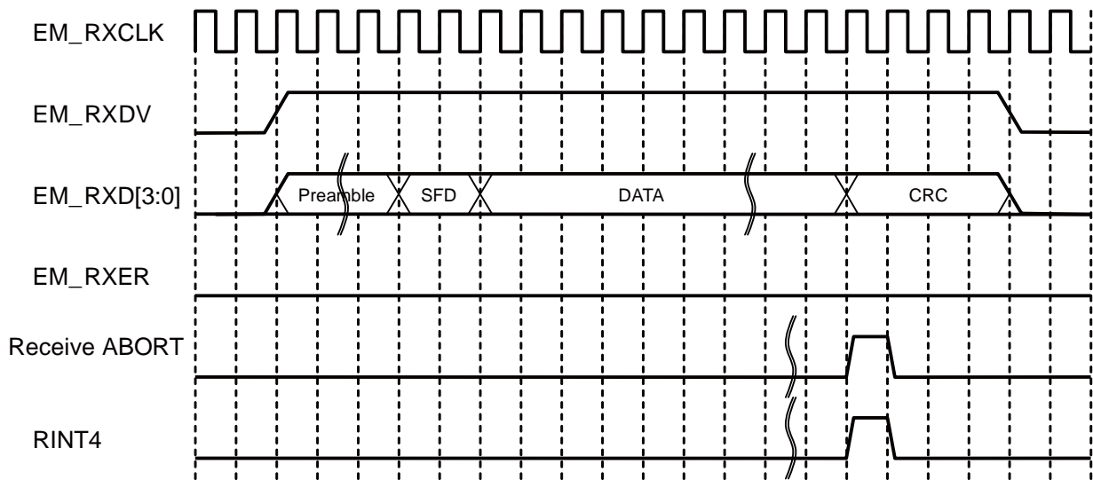
Figure 20-12 MII Frame Receive Timing (when a receive error and a long-frame error occur)
