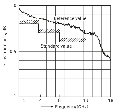
Insertion loss
