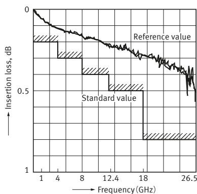
Insertion loss
