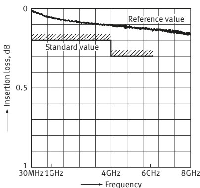
Insertion loss
