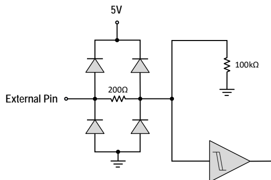
Figure 116. Internal Pull-down Configuration for the SPI_I3C_SEL, ID_0, and ID_1 Control Pins
