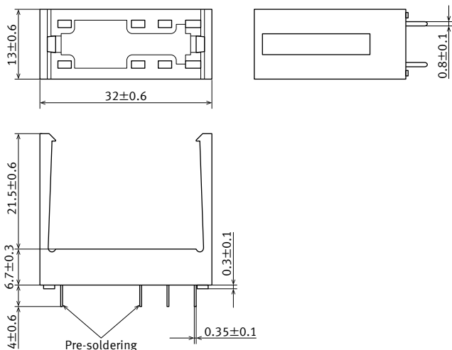
External dimensions
