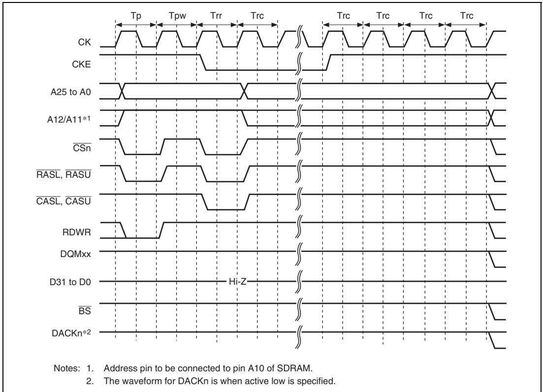
Figure 9.30 Self-Refresh Timing
