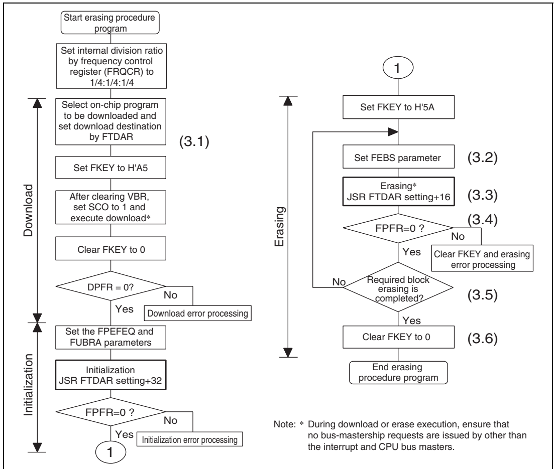
Figure 23.12 Erasing Procedure
