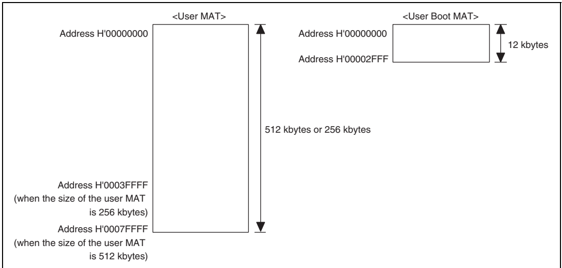
Figure 23.3 Flash Memory Configuration
