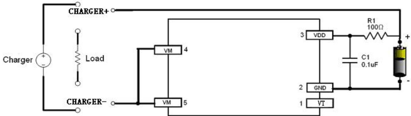
Fig 6 XB5353G in a Typical Battery Protection Circuit
