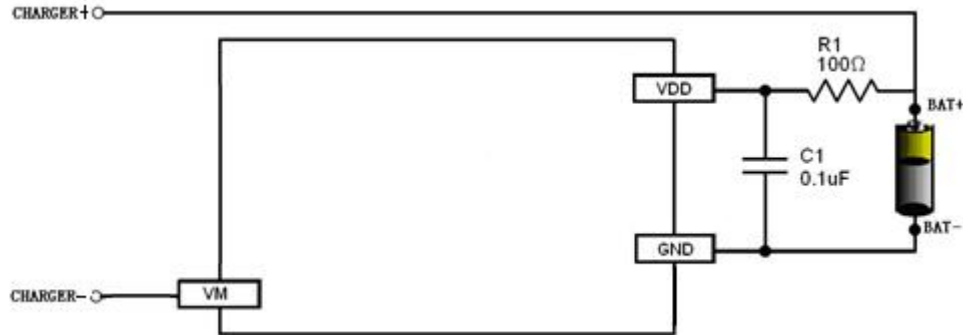
Fig 6 XB3301A in a Typical Battery Protection Circuit
