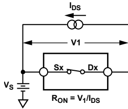
Figure 24. On Resistance
