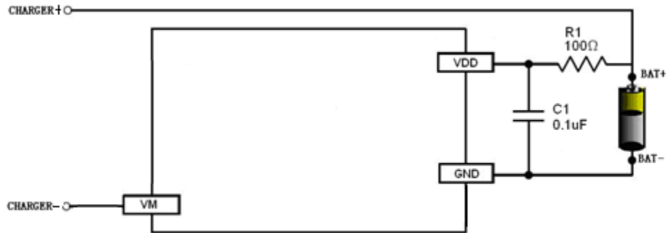
Fig 6 XB3301AJ in a Typical Battery Protection Circuit
