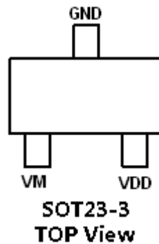
Figure 2. PIN Configuration
