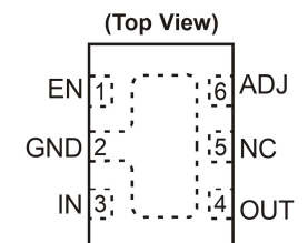
U-DFN2020-6 (ADJ Output) (SN Package)
