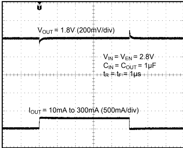
Load Transient Response Time (100µs/div)
