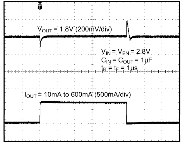
Load Transient Response Time (100µs/div)
