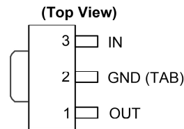
SOT89 (Fixed output) (Y Package)
