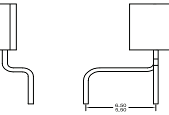
SOT54 LEAD BEND L02 Bulk Pack - 412
