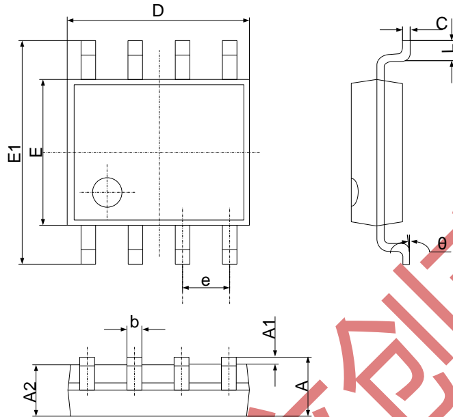
SOP-8
