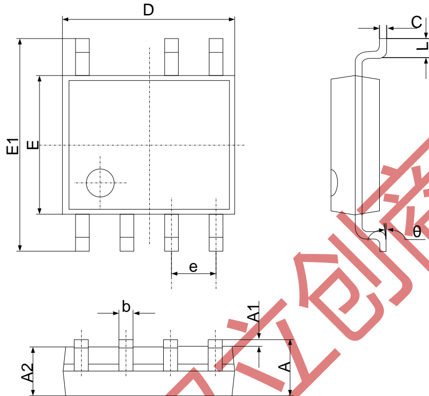
SOP-7
