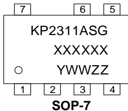
SOP-7
