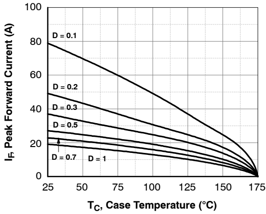
Figure 3. Current Derating
