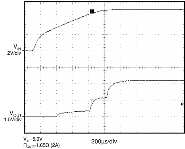
Start Up (Power up V_{IN} ) ( V_{OUT} = 3.3\text{V} )
