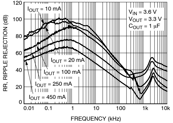
Figure 25. Power Supply Rejection Ratio, V_{OUT} = 3.3 V
