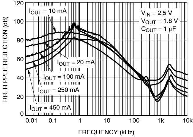
Figure 24. Power Supply Rejection Ratio, V_{OUT} = 1.8 V
