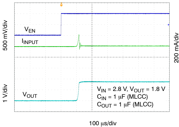
Figure 28. Enable Turn-on Response - C_{OUT} = 1 \mu F, I_{OUT} = 10 mA
