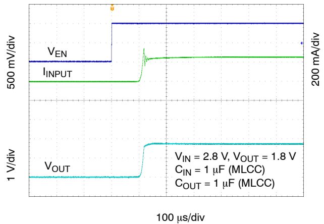
Figure 29. Enable Turn-on Response - C_{OUT} = 1 \mu F, I_{OUT} = 250 mA
