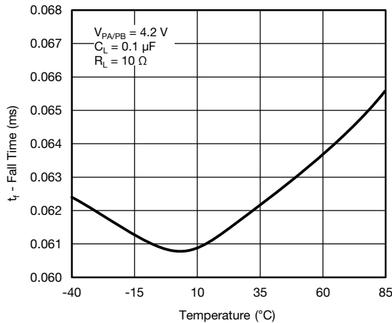
Fig. 18 - Port B Turn-On Time ( V_{PA} = 4.2 V , R_L = 10 \Omega , C_L = 0.1 \mu F )
