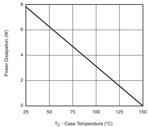
Power Derating
