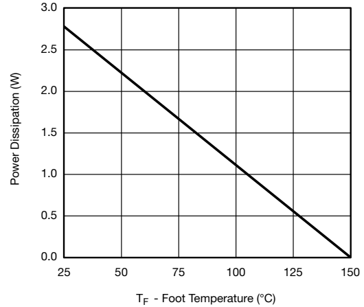
Power Derating
