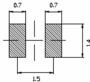
LAND PATTERN<REFERENCE>
