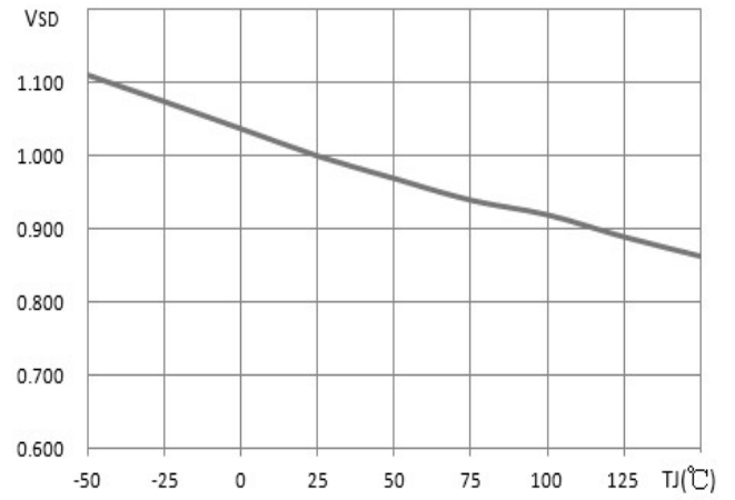
Normalized VSD vs. temperature
