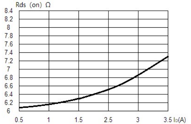
On-Resistance Variation vs. Id
