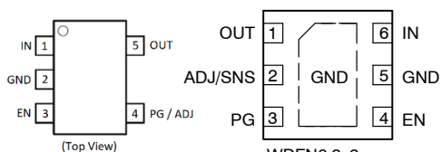
WDFN6 2x2 mm (Top View)
