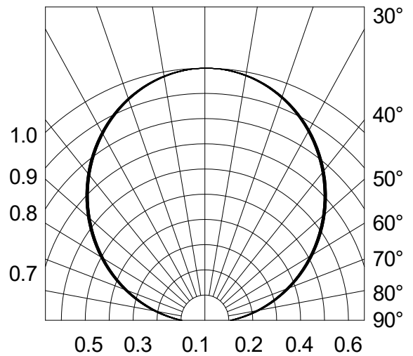
Fig.6-Radiation Diagram Ta=25°C
