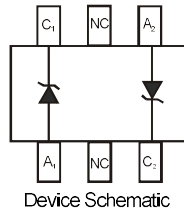
Device Schematic
