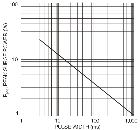
Fig. 6 Maximum Non-repetitive Surge Power
